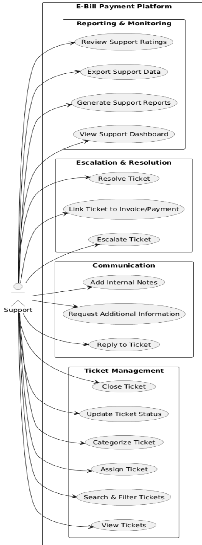
رسم توضیحي 6 Use Case Diagram: Support (Level 2)
