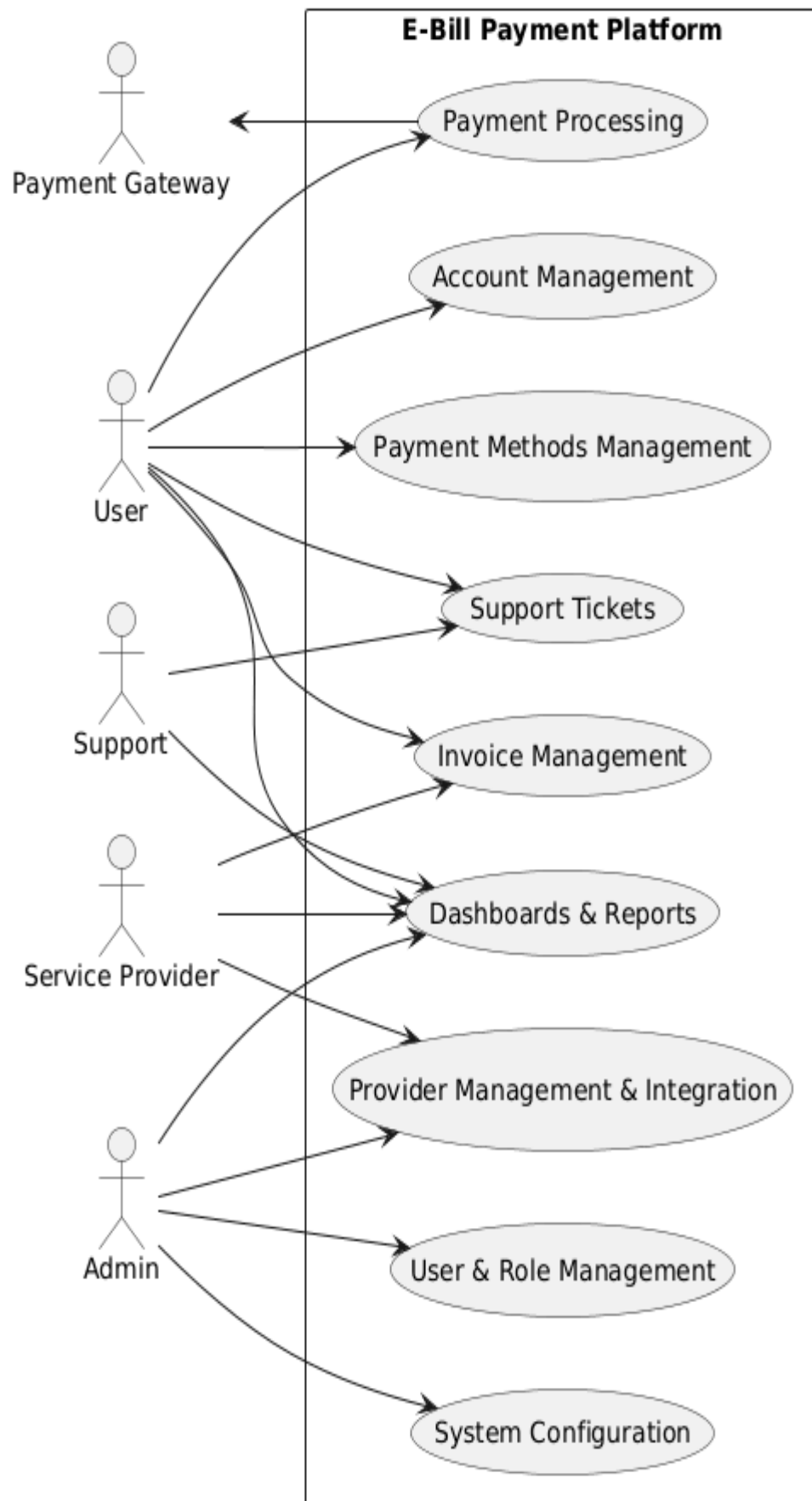
رسم توضیحي 2 High-Level Functional Use Case Diagram :
